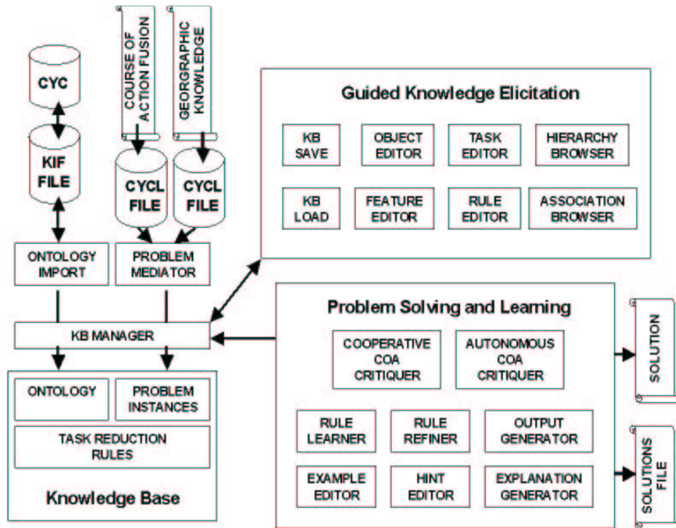
Figure 1. The Architecture of Disciple-COA
