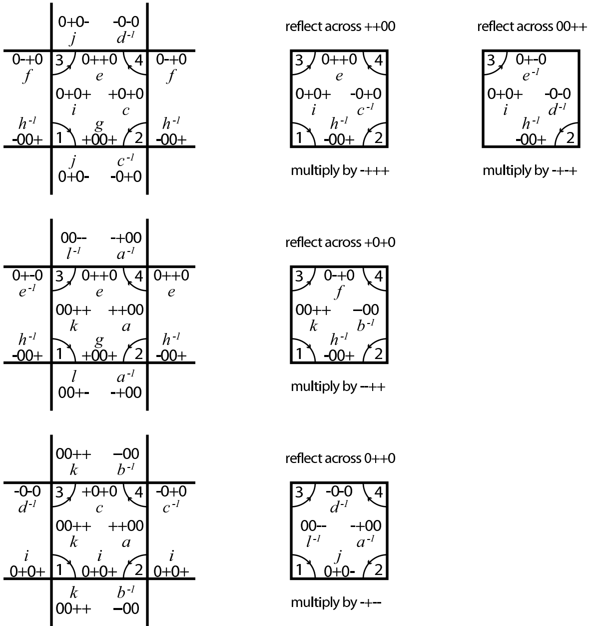
Figure 2: Diagrams that produce cycle relations for M_{56} .
