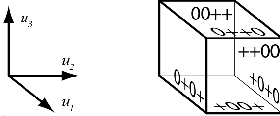
Figure 1: The cube Q_C when C is centered at v_{++++} .
