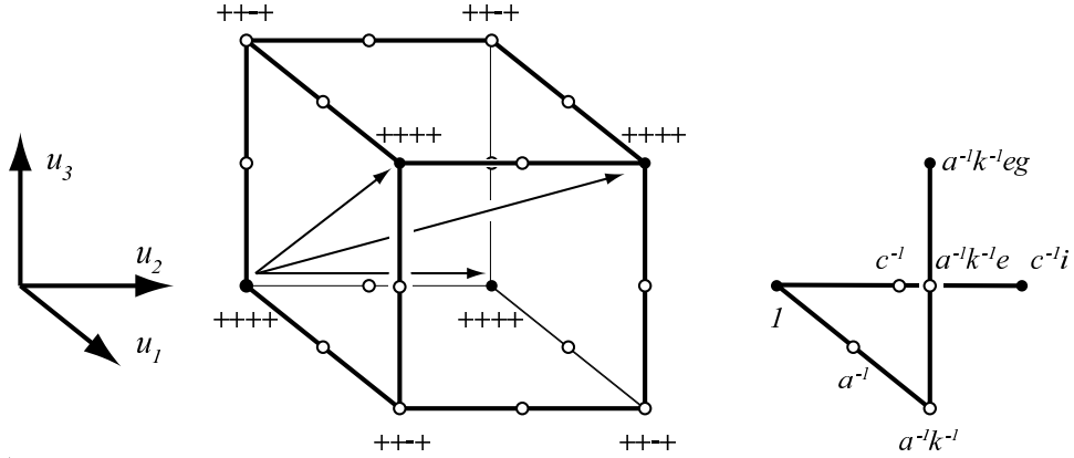
Figure 4: Translations in 64Q_C for manifold M_{56} .
